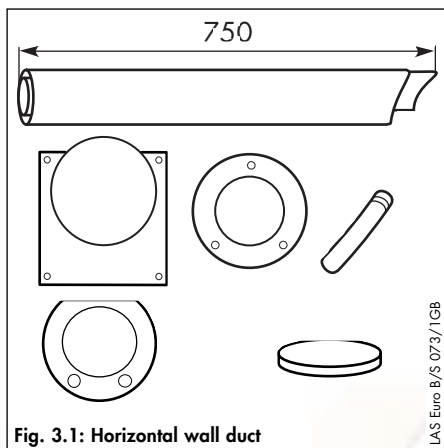
Fig. 3.1: Horizontal wall duct
